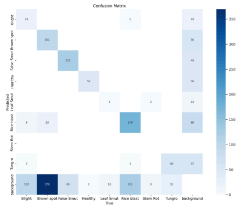
42 Fig. 3 – Confusion Matrix for Rice Disease Detection
