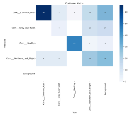
Fig. 5 – Confusion Matrix for Maize Disease Detection
