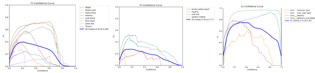
Fig. 12 – F1 Curve of Rice, Wheat, Maize Model's
