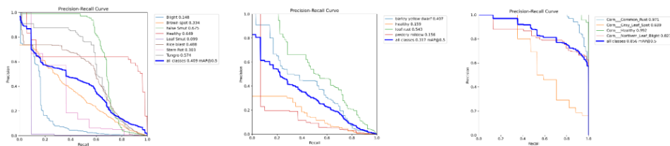
Fig. 11 – PR Curve (Precision-Recall Curve) of Rice, Wheat, Maize Model's
